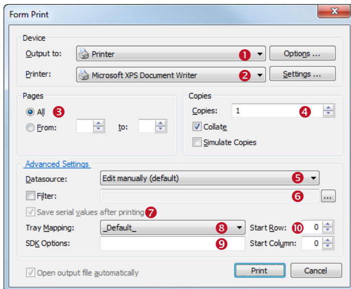
Figure 69: Print Dialog (with Advanced Settings enabled)
