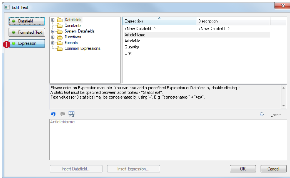
Figure 41: Edit Text Dialog – Expression
