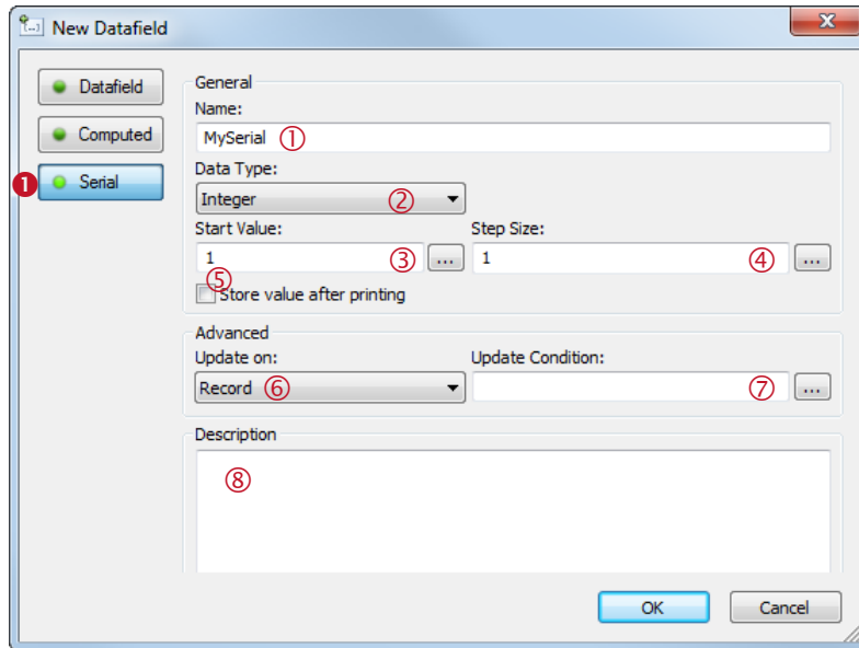
Figure 48: Edit Datafield Dialog – Serial Number
