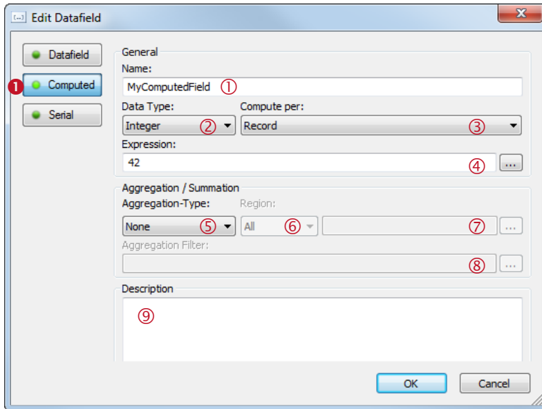
Figure 46: Edit Datafield Dialog – Computed
