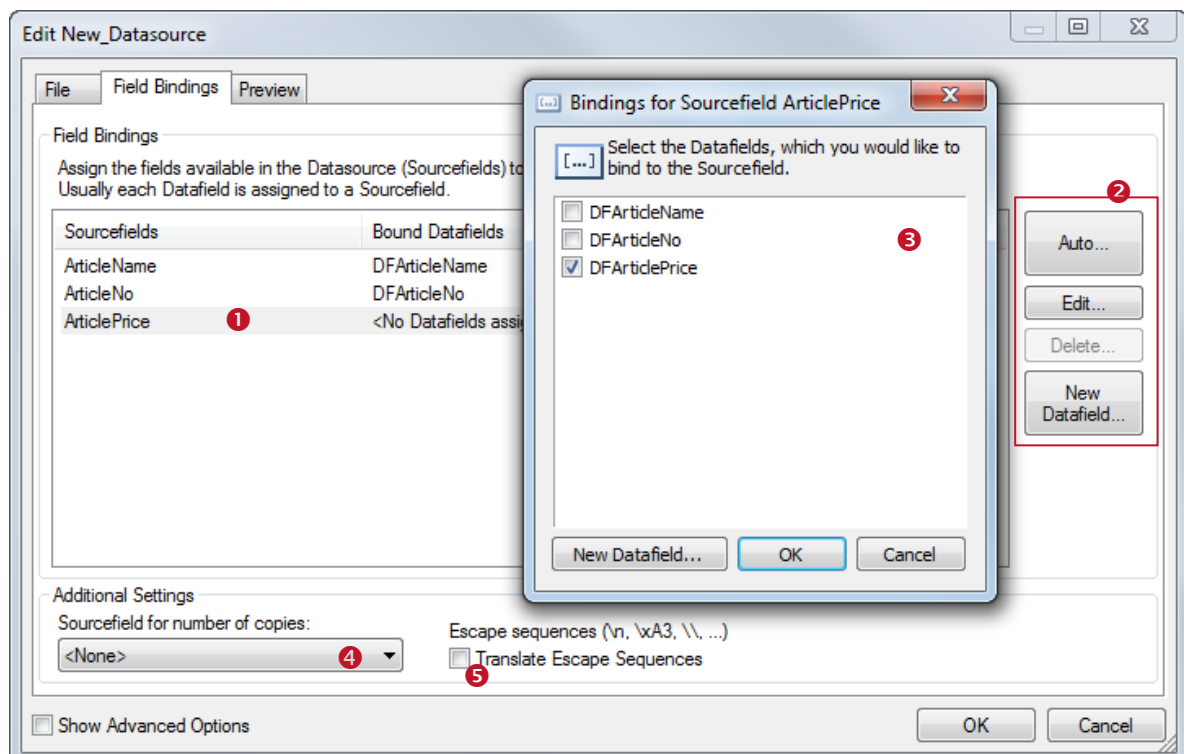
Figure 58: Field Bindings Settings
