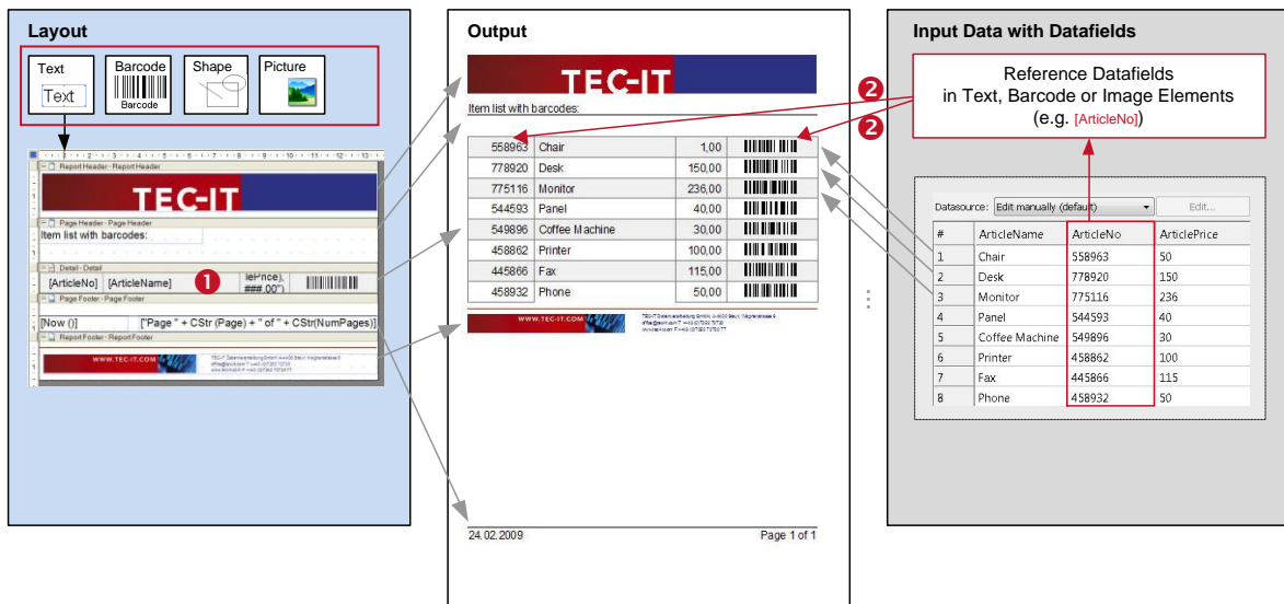
Figure 42: Datafields as Part of the Printing Concept
