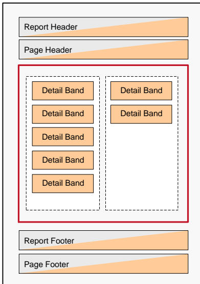
Figure 74: Report with Columns
