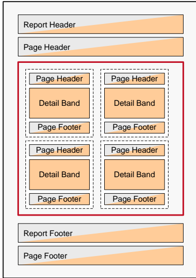
Figure 78: Label Sheets with Headers and Footers
