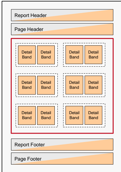
Figure 81: Label Sheets with Detail Band Columns
