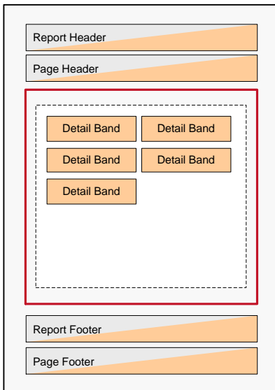
Figure 80: Report with Detail Band Columns
