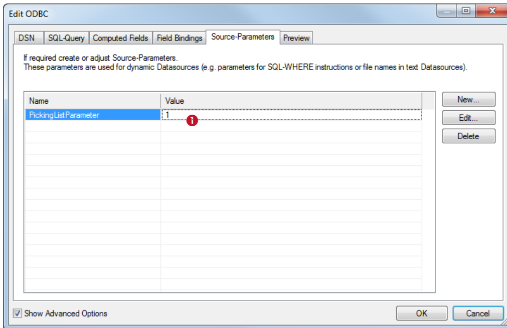
Figure 63: Edit a Source-Parameter Value
