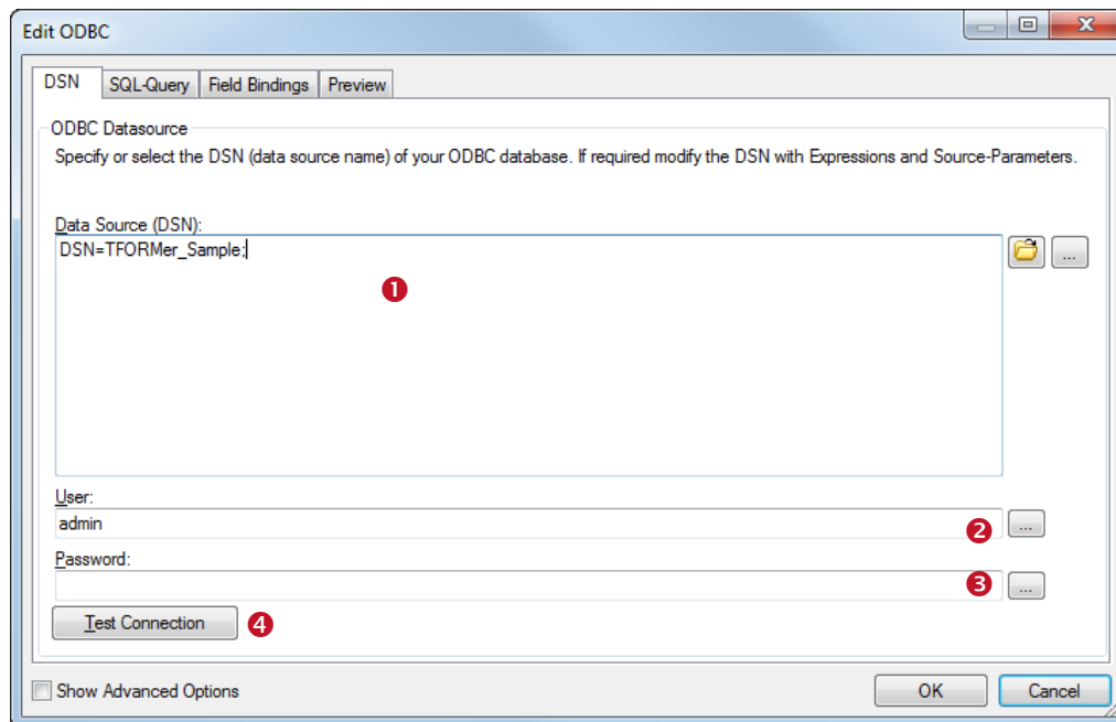
Figure 54: Data Source (DSN)
