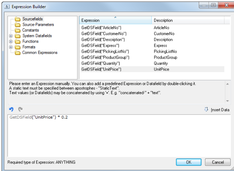
Figure 60: Example of an expression for a computed field
