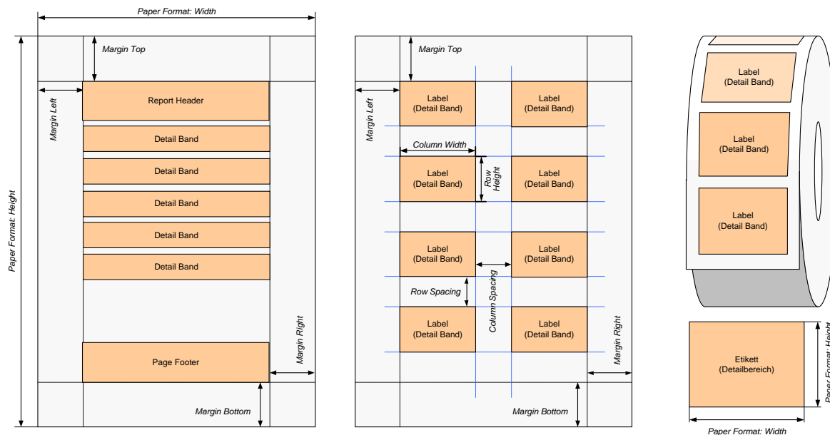
Figure 26: Page Setup for Standard Reports, Label Sheets, and Label Printers
