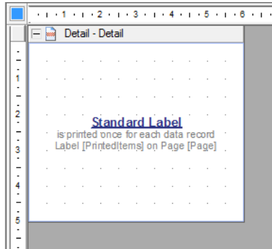
Figure 23: Label Printer – Layout View
