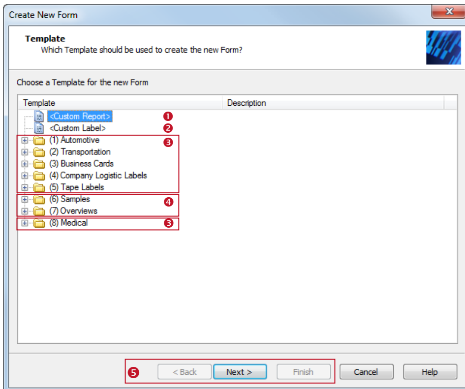
Figure 15: Create a New Layout
