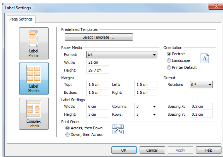
Figure 32: Page Setup
