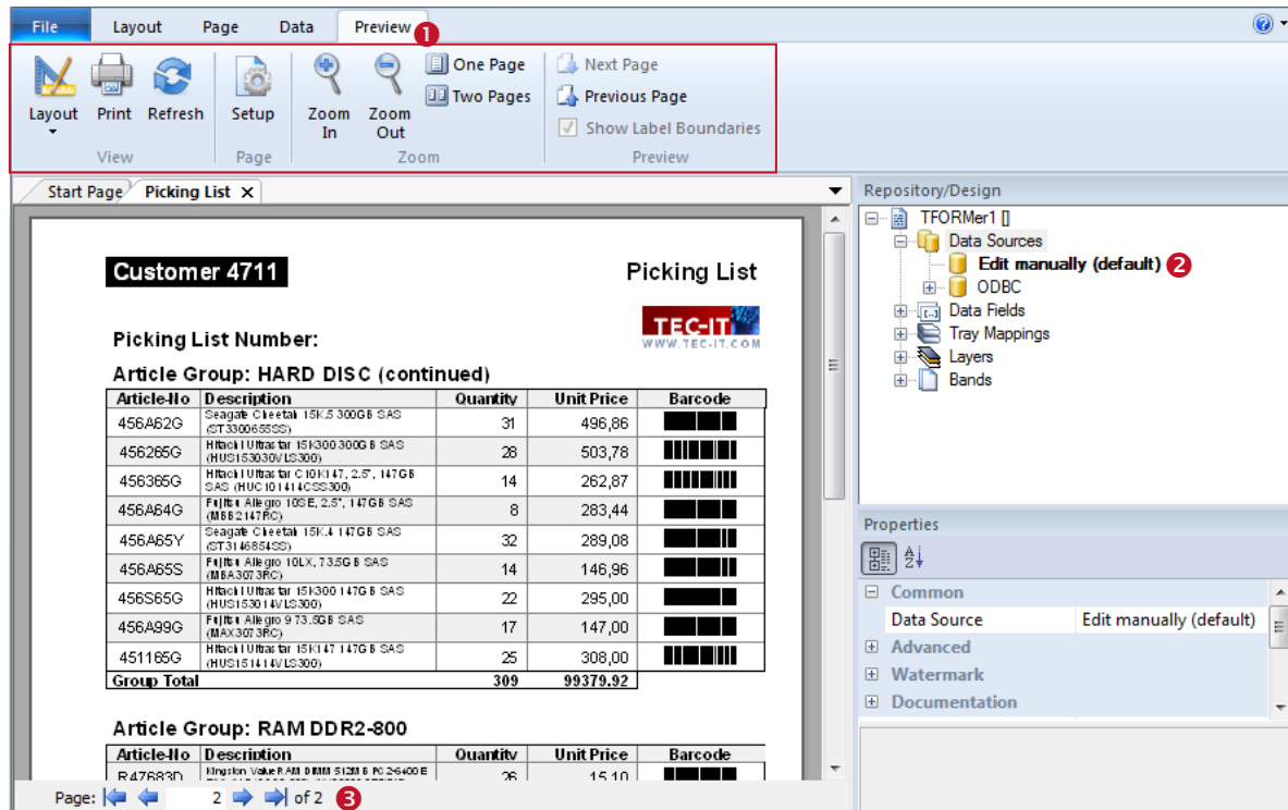
Figure 85: Preview
