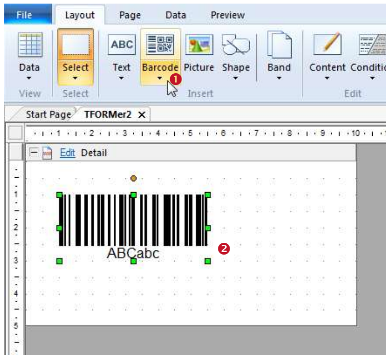
Figure 37: Insert Element
