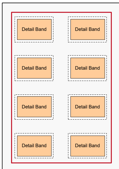
Figure 94: Label Sheets
