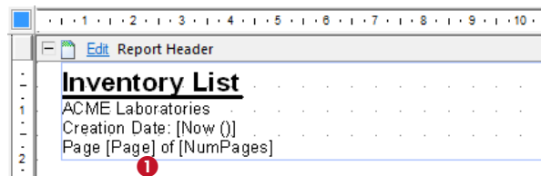
Figure 39: Text Element
