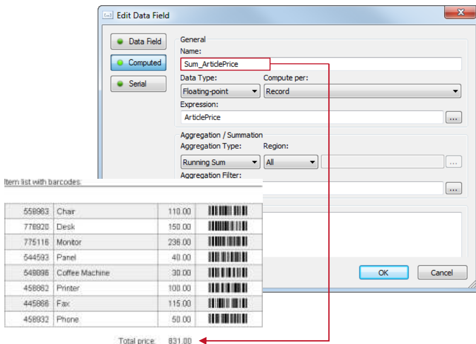
Figure 55: Calculate Sum
