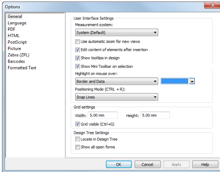
Figure 88: Options Dialog
