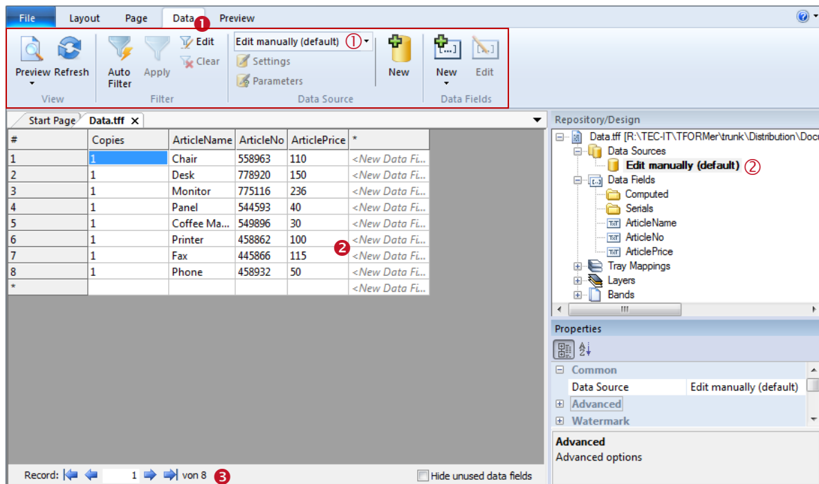
Figure 63: Data View
