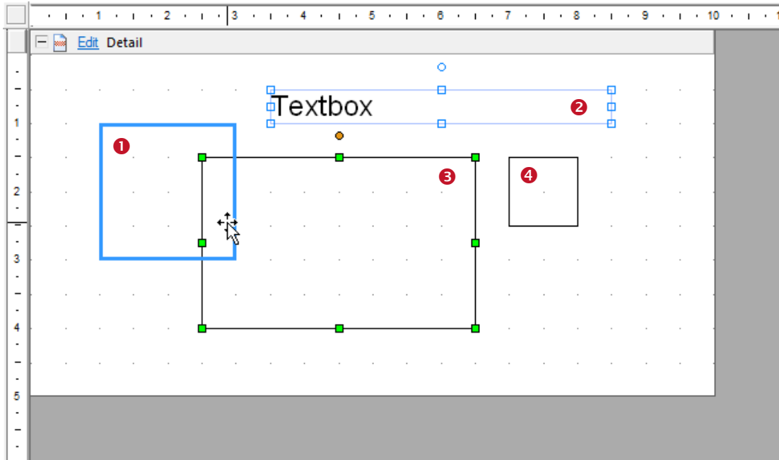
Figure 38: Element Selection
