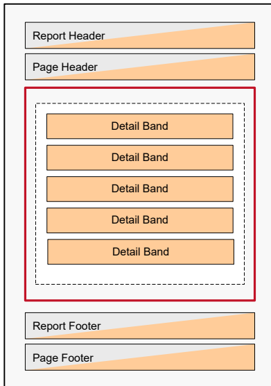
Figure 91: Simple Report
