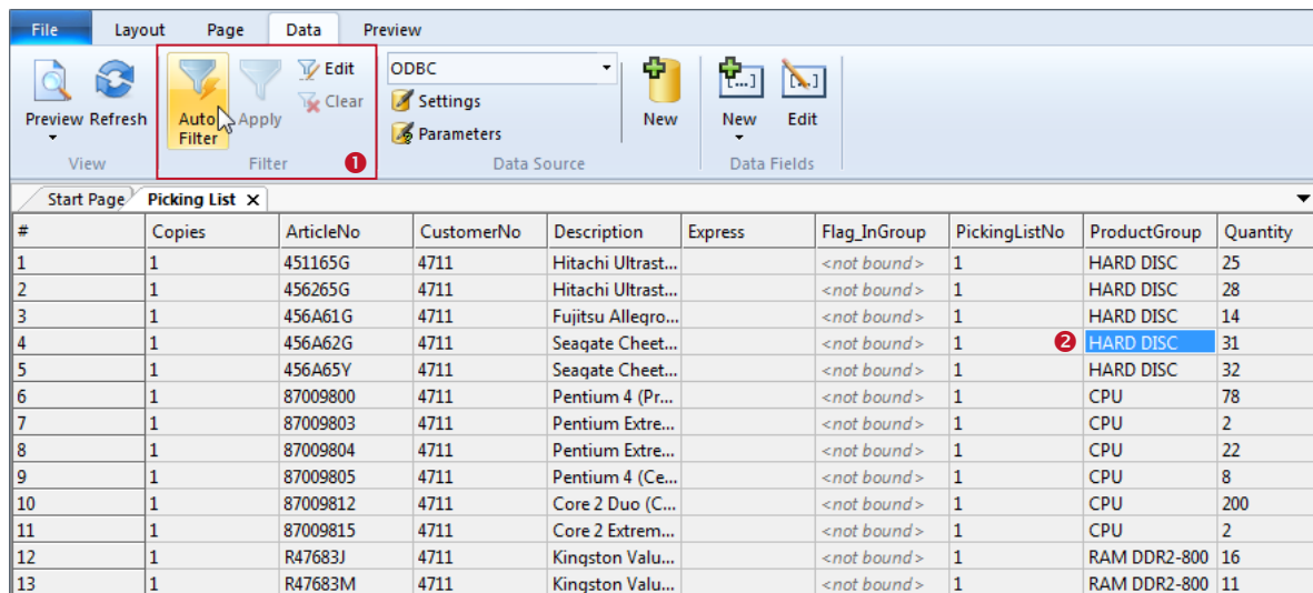
Figure 81: Filter
