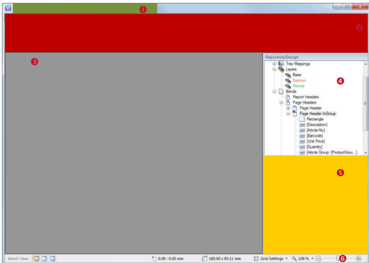
Figure 2: User Interface
