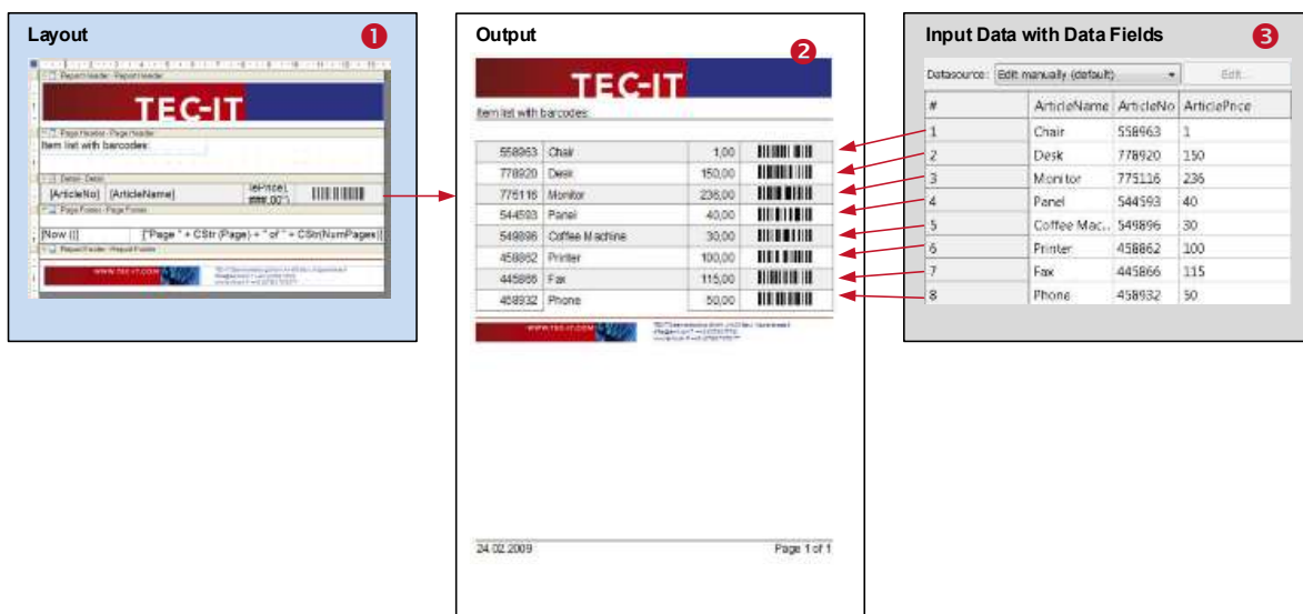
Figure 19: Printing Concept
