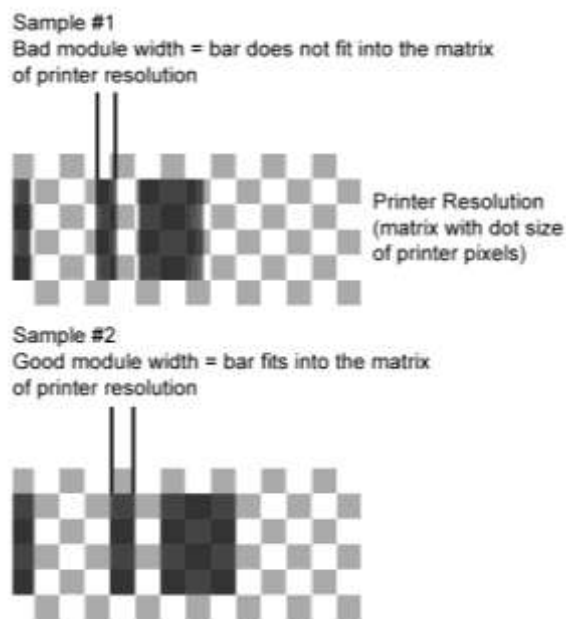
Figure 6: Raster Optimization
